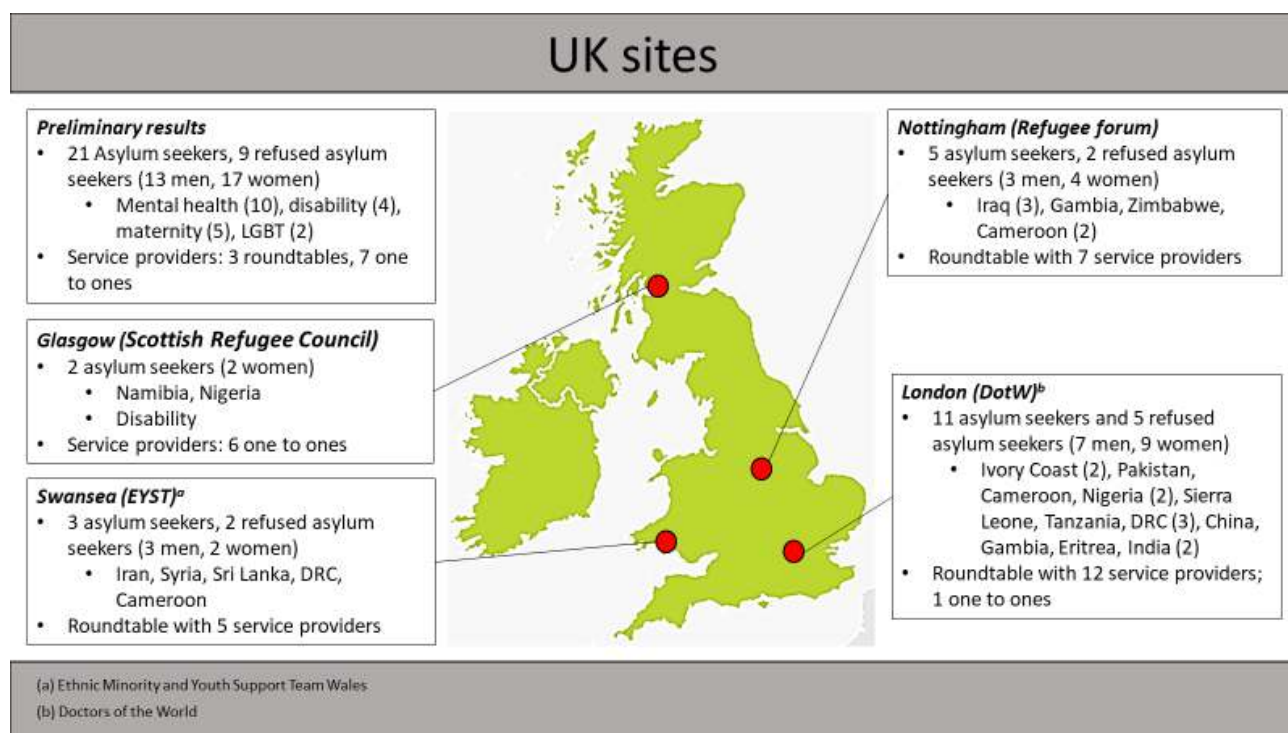
Figure 1 Fieldwork sites
